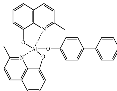
BAQ
