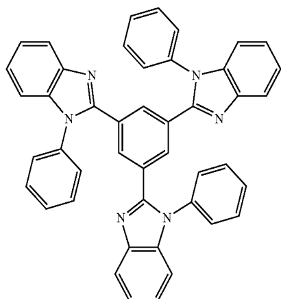
TPBi
