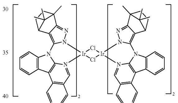
Compound M1B
