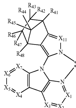
Formula 11-2
