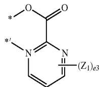
Formula 3-1
