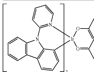
Comparative Compound 1
