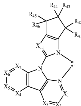
Formula 11-3
