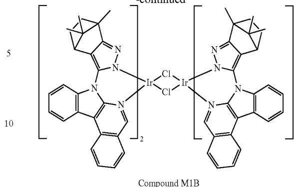
Compound M1B
