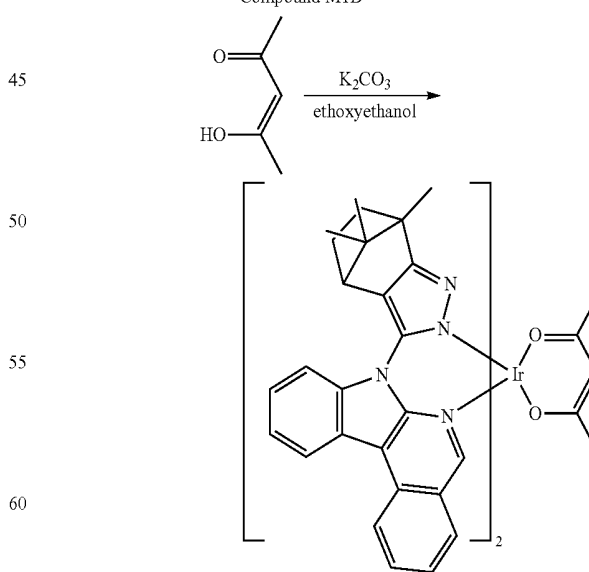
Compound 19
