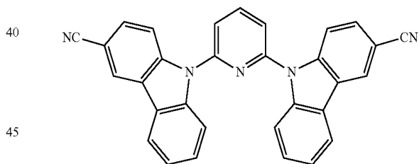
Compound H51
