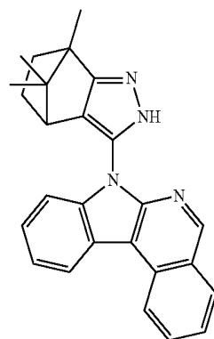
Compound B
