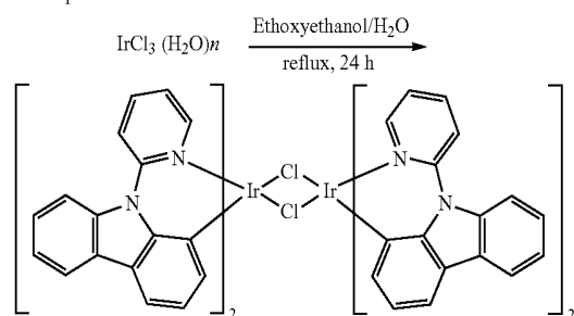
Compound M1C
