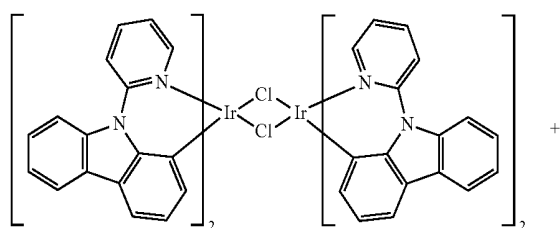
Compound M1C
