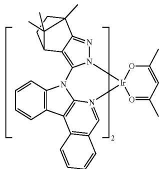
Compound 19
