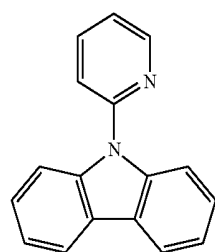
Compound C
