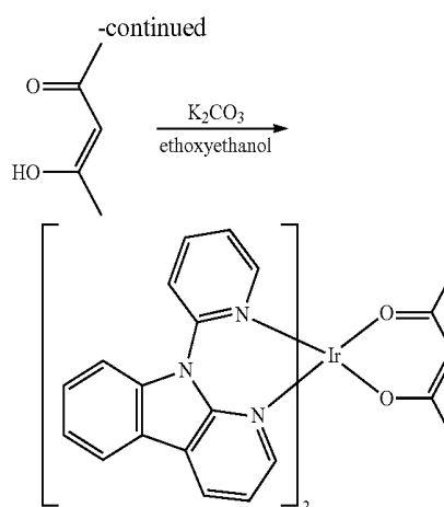
Comparative Compound 1
