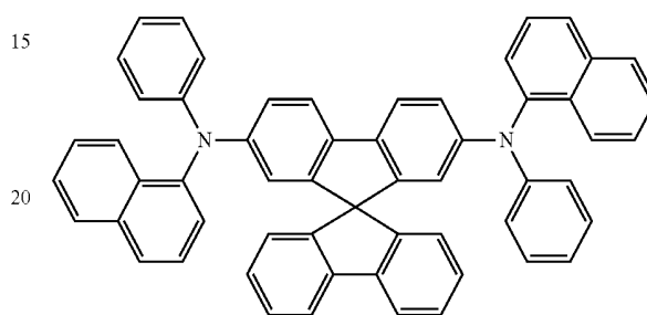
Spiro-NPB
