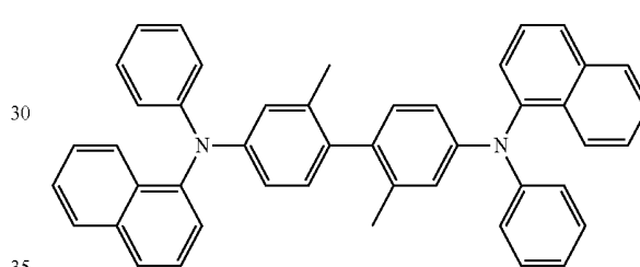
methylated NPB
