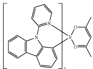
Comparative Compound 1
