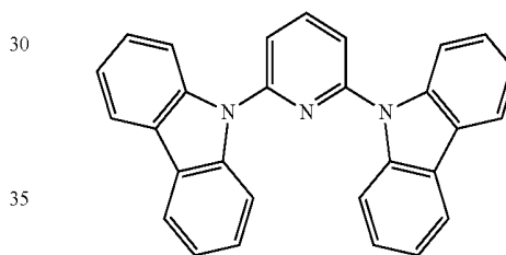
mCP
